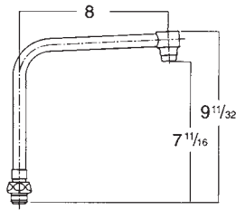
#HA8 E12 aerator Special order
