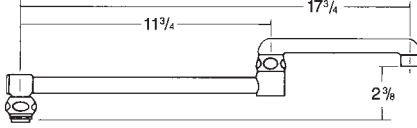
DJ18 E3 aerator, E2 outlet available Special order
