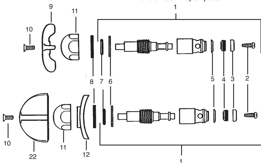
Flo-Cloz stem repair parts
