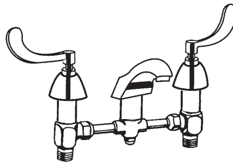
Deck mounted fitting. 5" spout. E12 Softflo aerator. Wrist blade handles and Quaturn operating cartridge.
